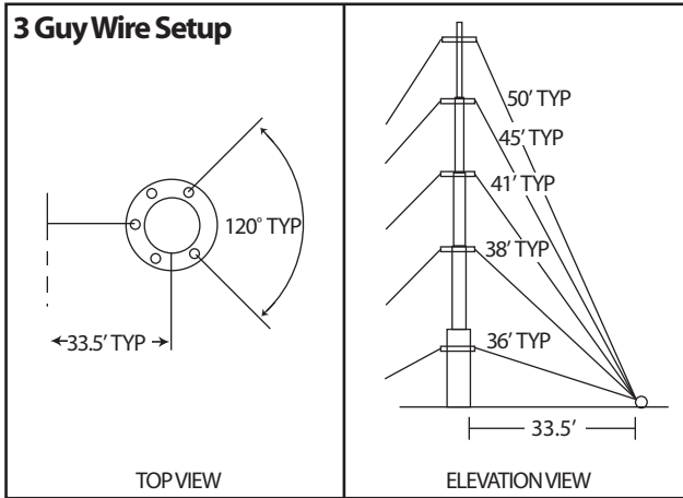
9H503WAYGUY
