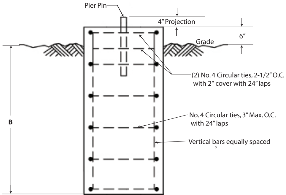
ELEVATION VIEW
