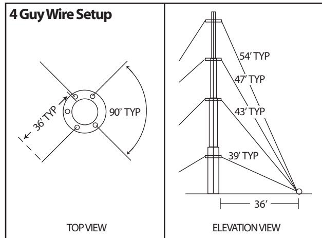
H404WAYGUY
