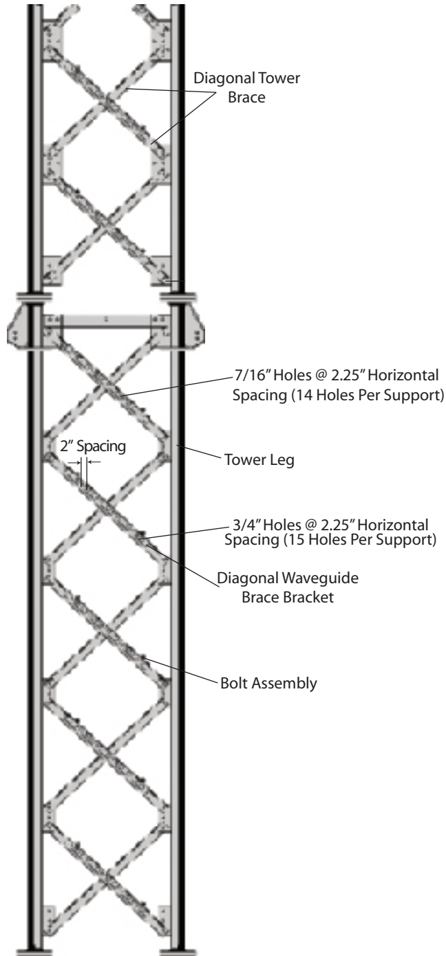
Angle Bracing
