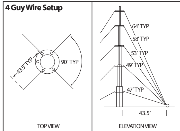
H504WAYGUY
