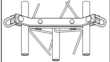
GUY BRACKET GA55GD MOUNTS TO TOWER AT ANY HORIZONTAL BRACE.
