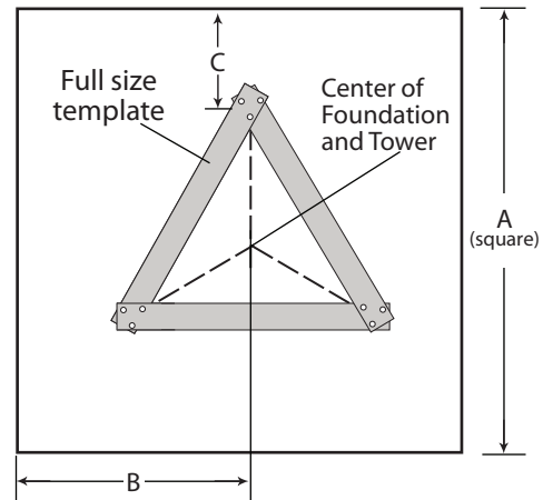
ANCHOR BASE
