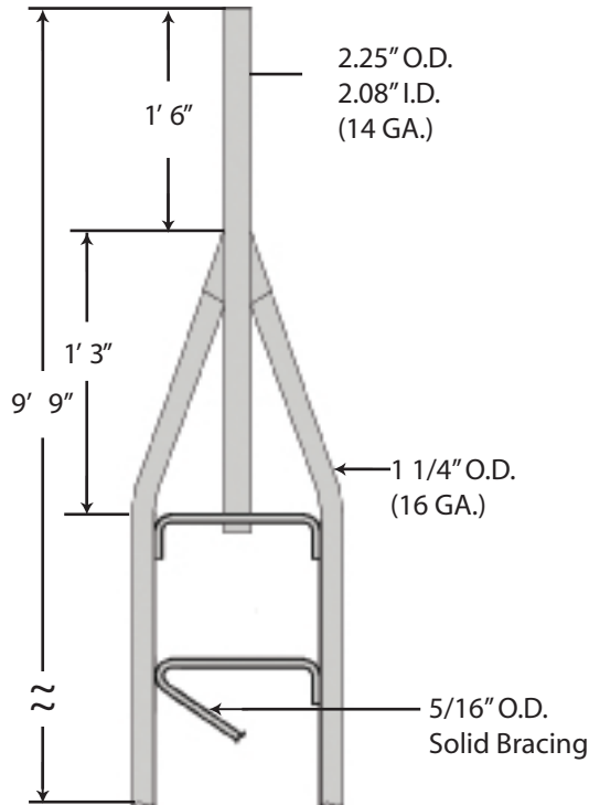
STANDARD TOP SECTION 25AG2
