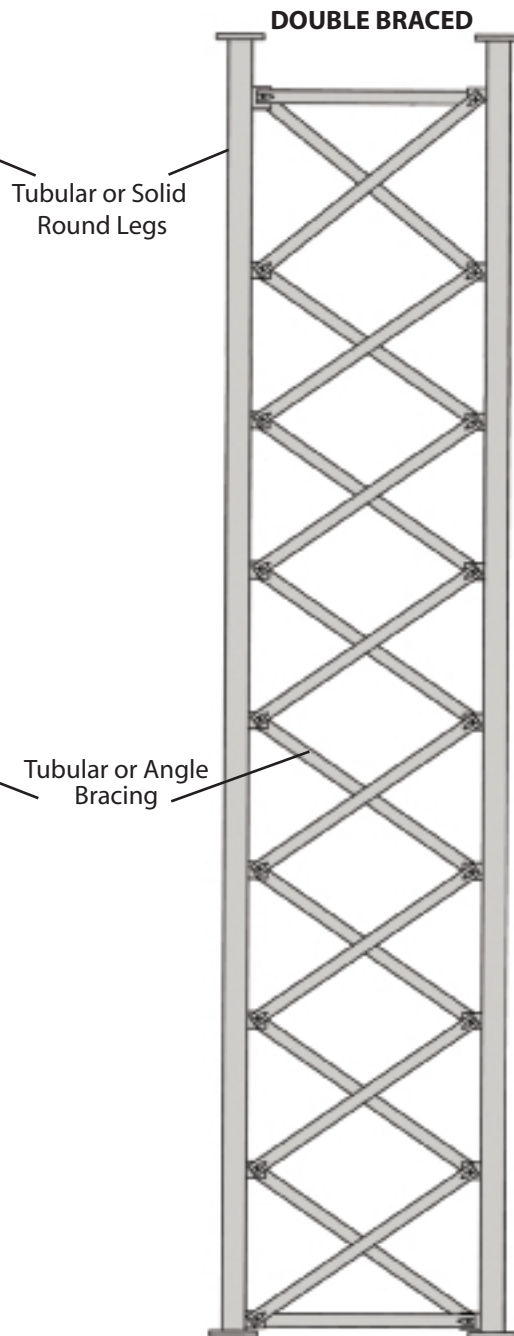
20' STANDARD SECTION
