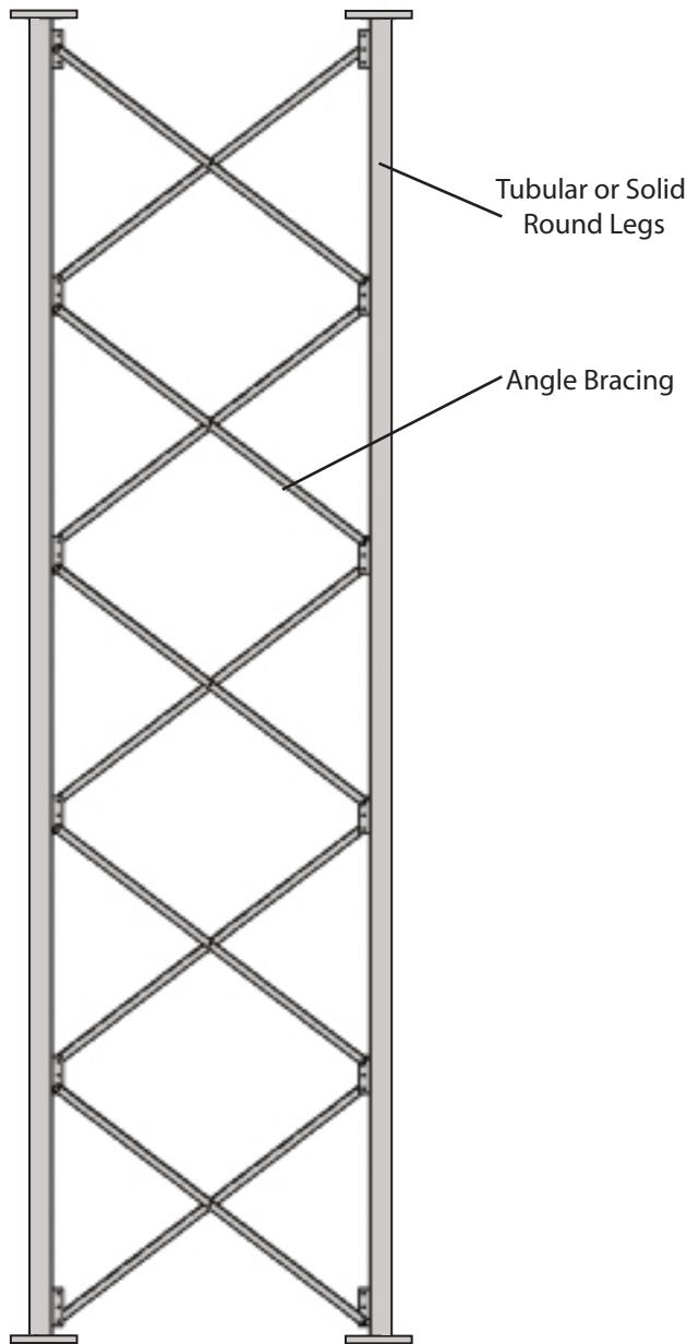
ELEVATION 20' STANDARD SECTION
