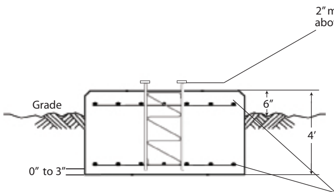
ELEVATION VIEW 45GSR SELF-SUPPORTING TOWER FOUNDATION
