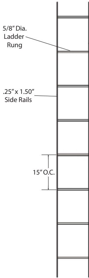
STANDARD LADDER NL10 - 10' ladder NL20 - 20' ladder
