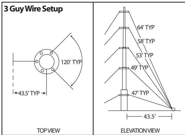
H503WAYGUY
