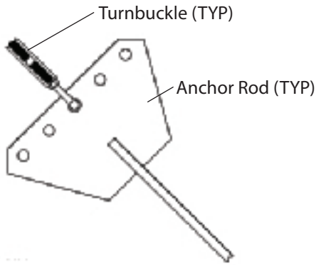
1 Guy Attachment
