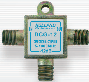
MODEL DCG-*
